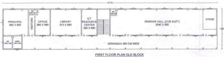
FIRST FLOOR PLAN OLD BLOCK
