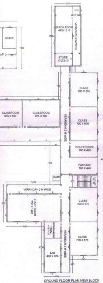
GROUND FLOOR PLAN NEW BLOCK
